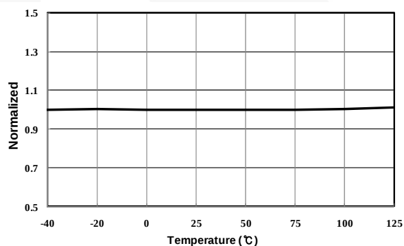
Figure 8. V_{DD-OVP} vs. Temperature
