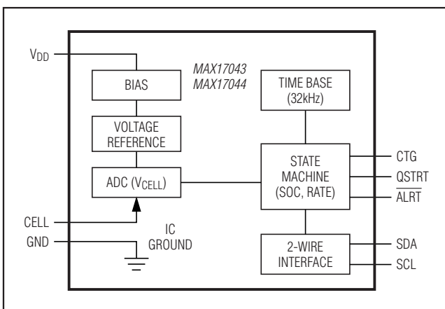
Figure 2. Block Diagram
