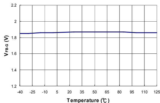
Figure 13. Green-Mode Ending FB Voltage ( V_{FB-G} ) vs. Temperature
