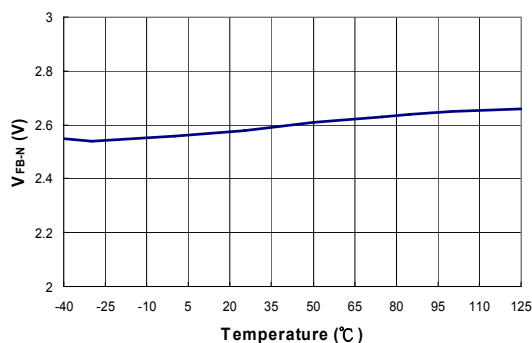
Figure 12. Green-Mode Entry FB Voltage ( V_{FB-N} ) vs. Temperature
