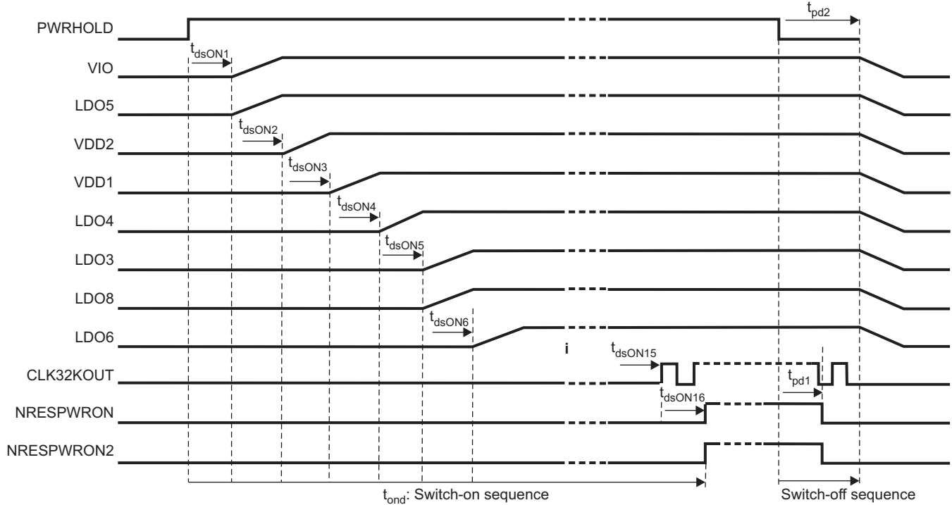
Figure 6-1. Boot Sequence Example with 2-ms Time Slot and Simultaneous Switch-Off of Resources
