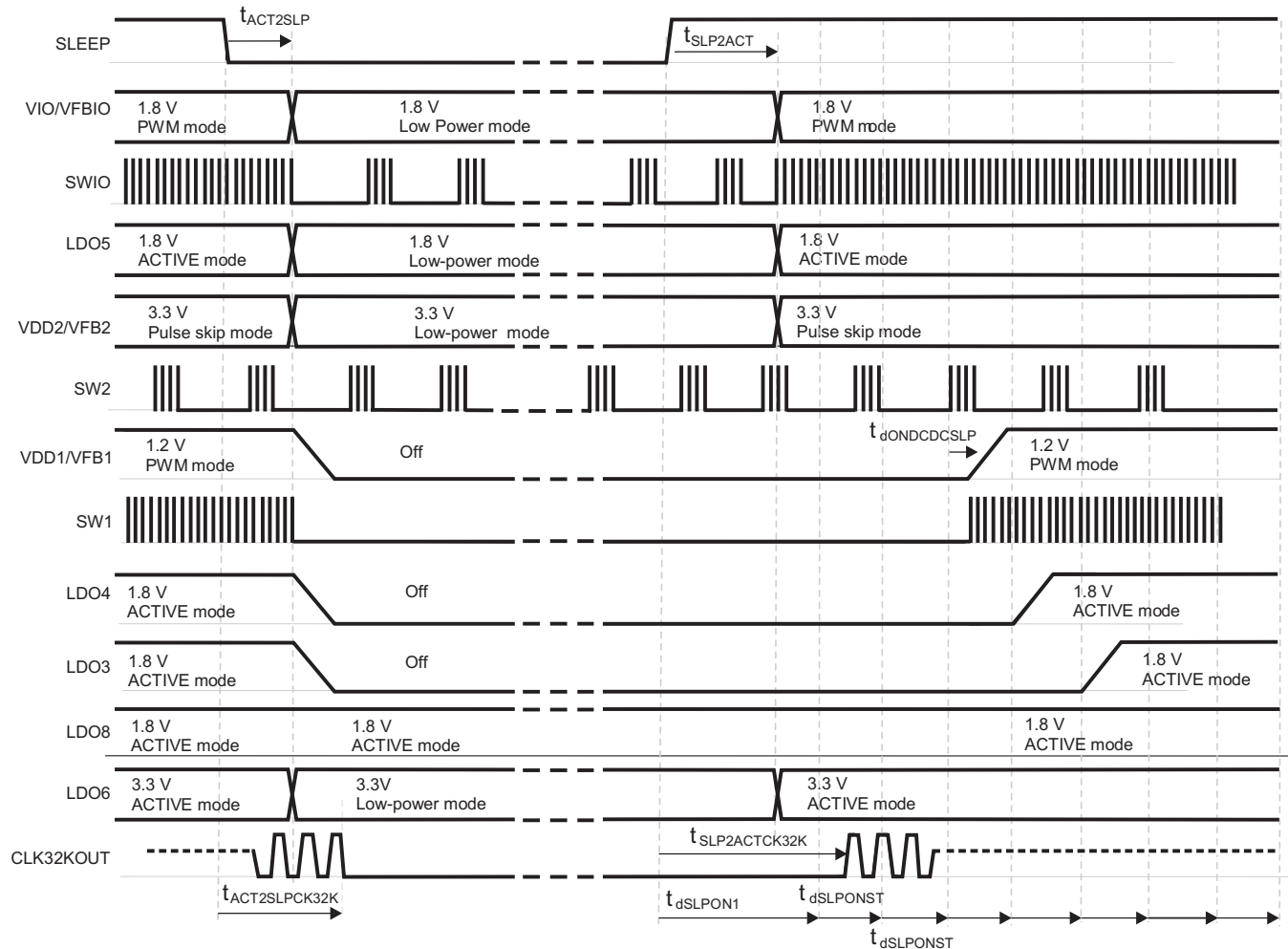
Figure 7-3. Device SLEEP State Control
