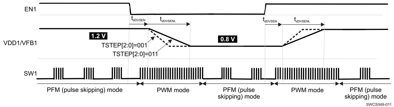
Figure 7-7. VDD1 Supply Voltage Control Through EN1
