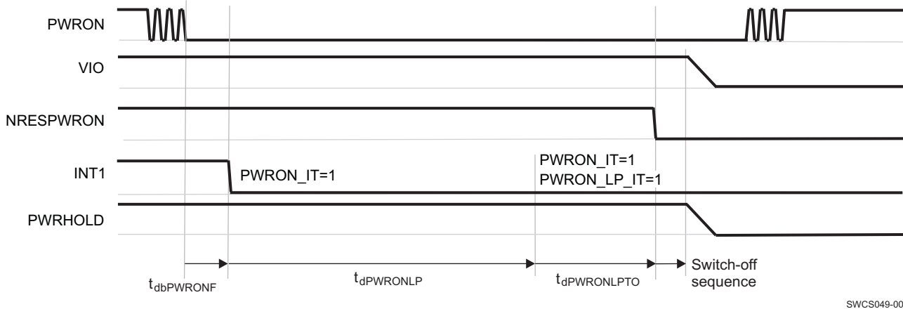
Figure 7-2. PWRON Long-Press Turn-Off
