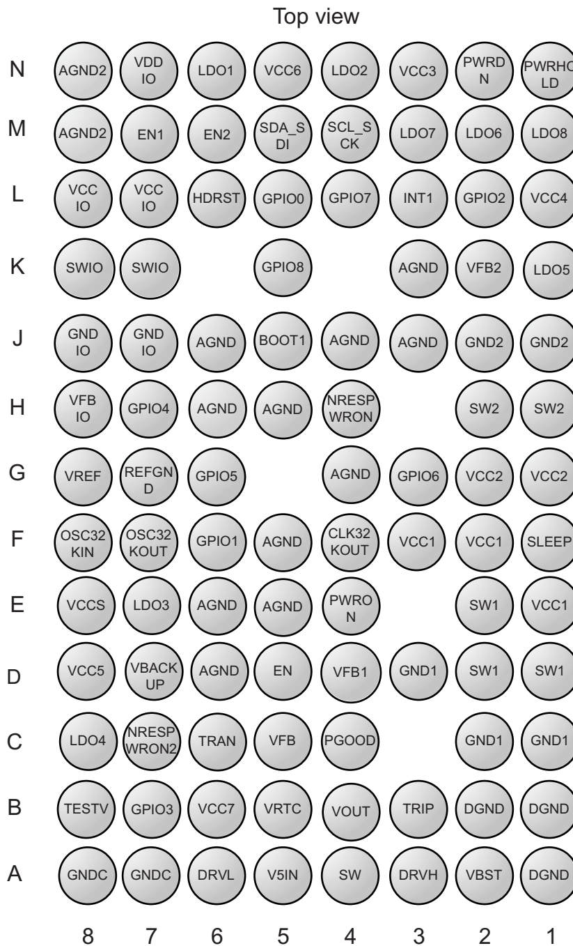
Figure 4-1. Ball Assignment - Top View
