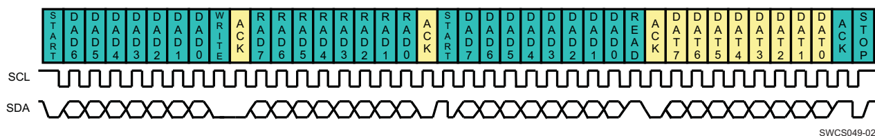
Figure 8-8. I 2 C Read Access Single Byte
