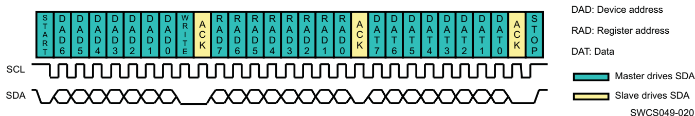
Figure 8-7. I 2 C Write Access Single Byte
