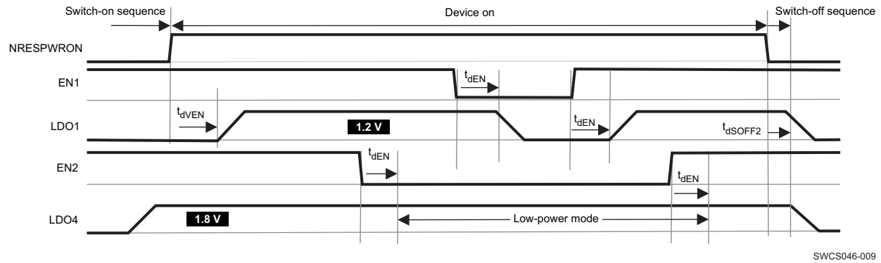
Figure 7-5. LDO Type Supplies State Control Through EN1 and EN2
