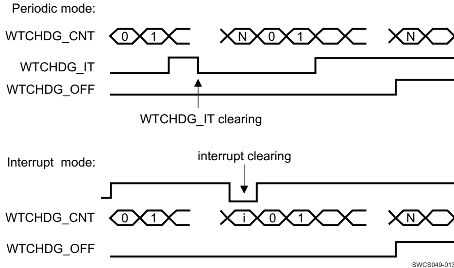
Figure 8-2. Watchdog Signals
