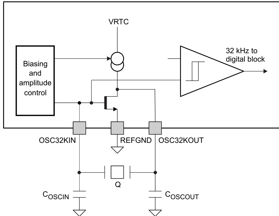
Figure 8-4. Crystal Oscillator 32-kHz Clock
