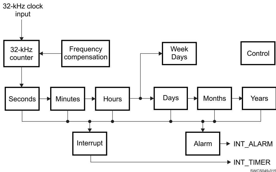
Figure 8-5. RTC Digital Section Block Diagram
