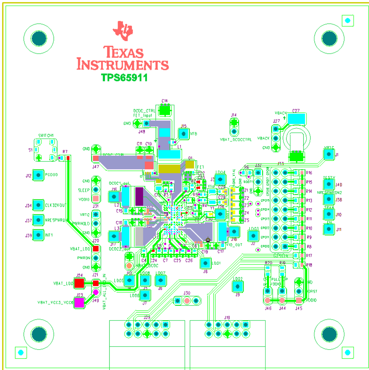
Figure 10-1. TPS65911 EVM Top Copper with Component Placement
