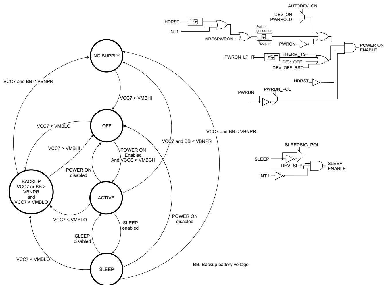
Figure 8-1. Embedded Power Control State-Machine
