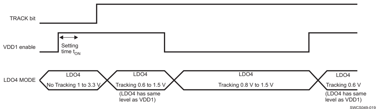
Figure 8-3. Tracking LDO
