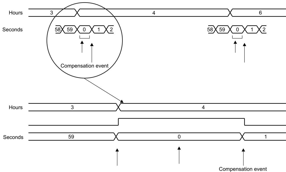
Figure 8-6. RTC Compensation Scheduling
