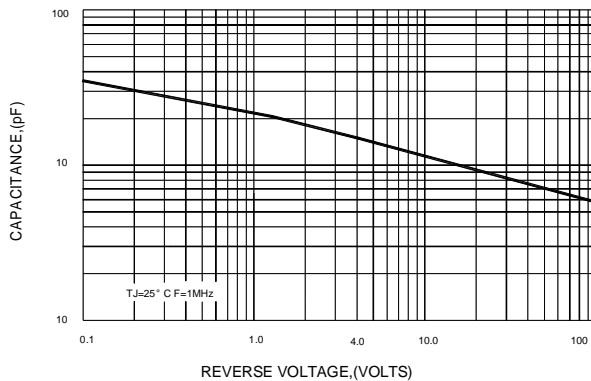
FIG.5-TYPICAL JUNCTION CAPACITANCE
