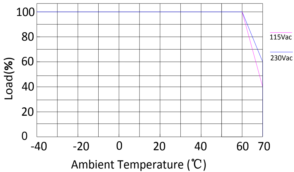
Derating Curve
